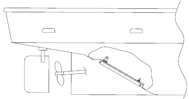
FIG. 3 Recessed installation is made by welding in a box-shaped recess in the underside of the hull. Note aft end of recess is tapered to prevent hot water entrapment.
