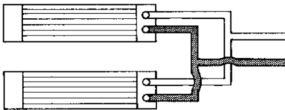
FIG. 14 Multiple-pass coolers connected in parallel
