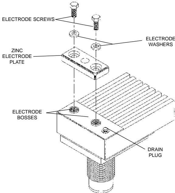
FIG. 11 Zinc Attachment Detail
