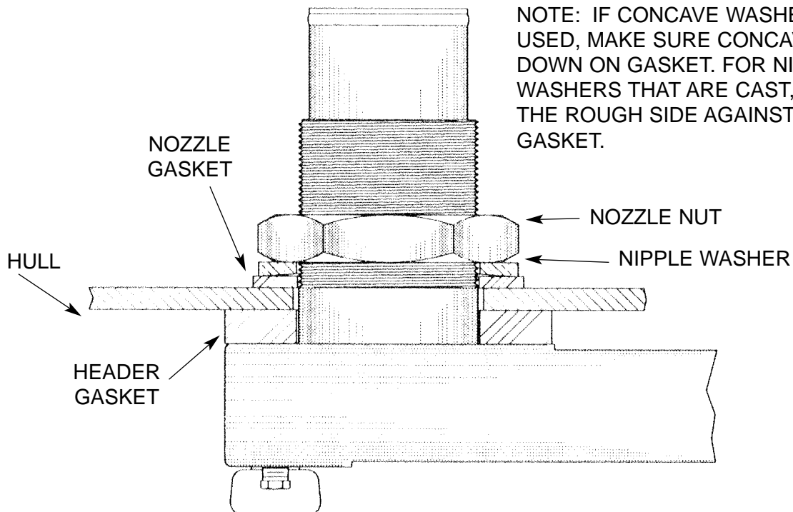
FIG. 10 Mounting Parts Placement
