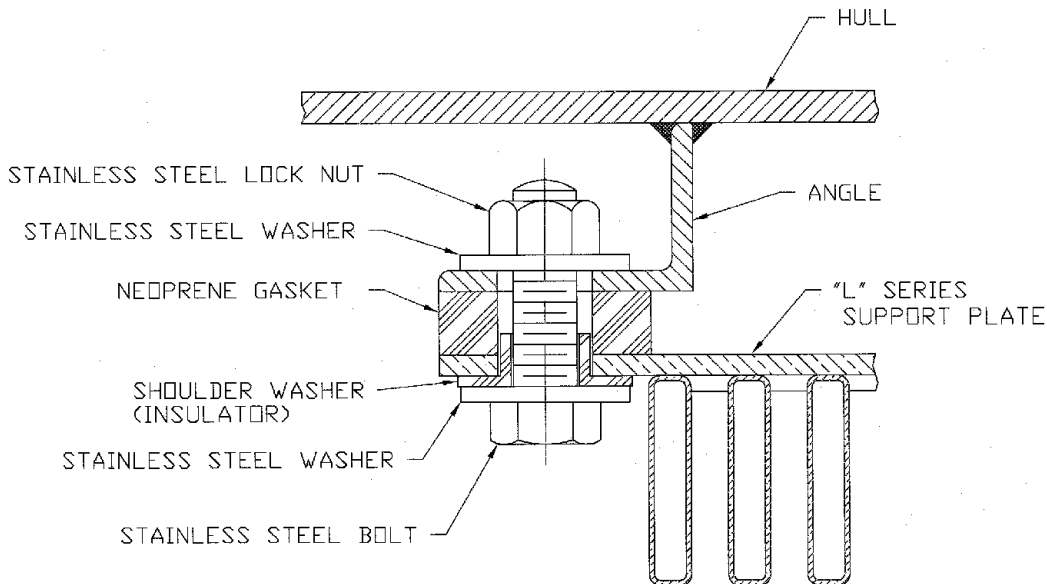
FIG. 22 L SERIES support plate with angle welded to hull
